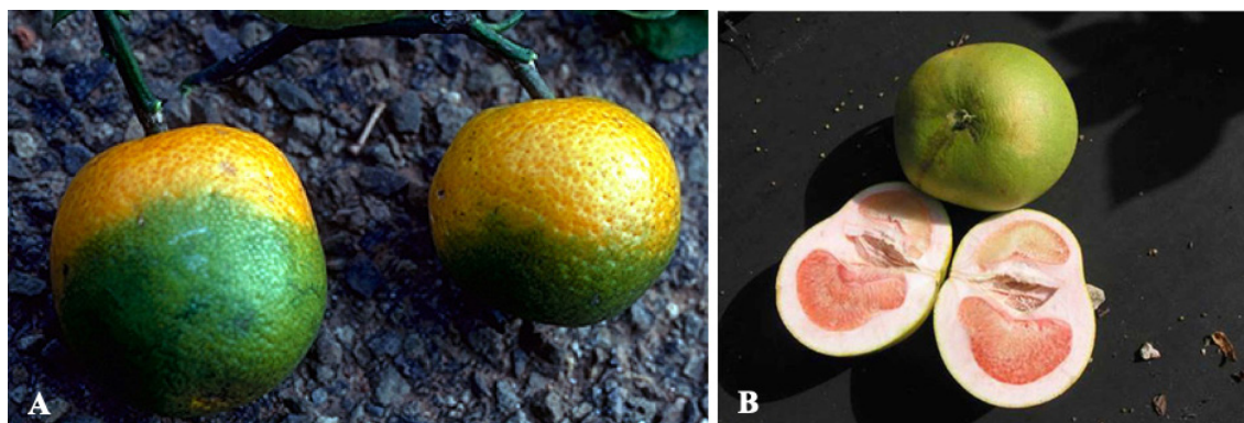
Figure 5. (a) Abnormal ripening of Citrus reticulata fruit infected with citrus huanglongbing; (b) cross section of misshapen Citrus x paradisi fruit infected with citrus huanglongbing
