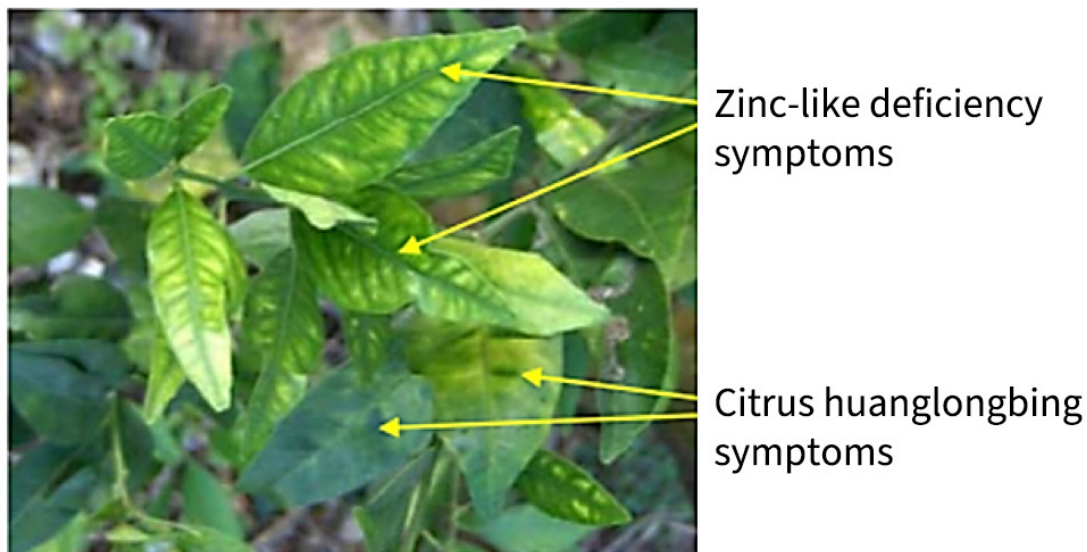
Figure 4. Zinc-like deficiency symptoms and classic citrus huanglongbing symptoms
